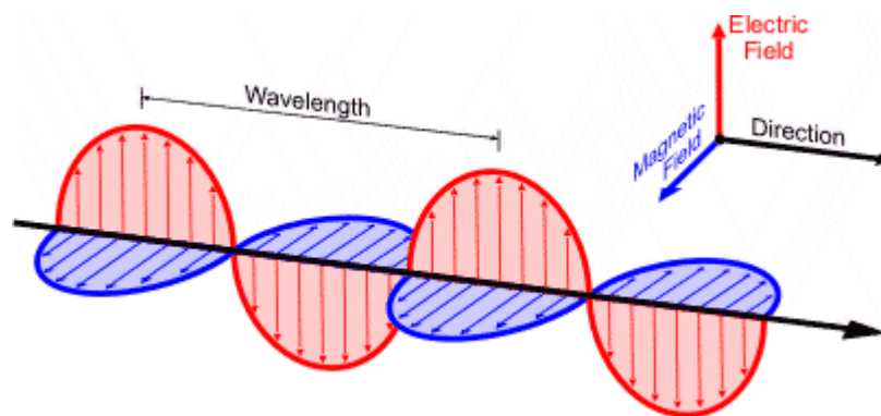
Figure 2 Electromagnetic waves
